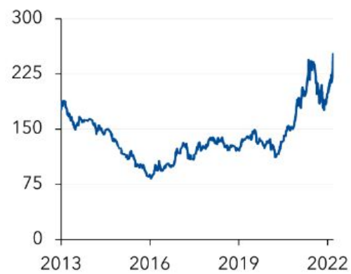
Metals Index** (2016=100)
